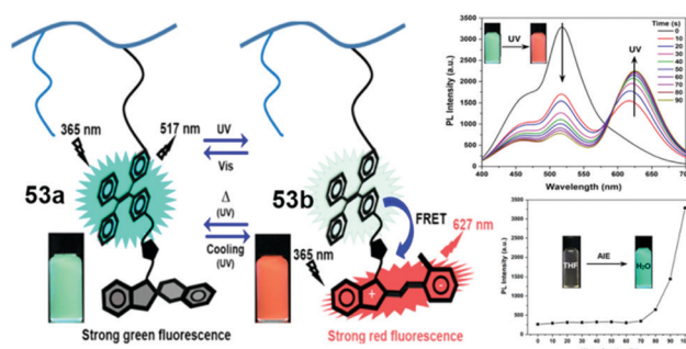
Fig. 24 Schematic illustration of the energy transfer from the TPE to MC unit via the FRET process after UV exposure and the AIE property of 53a in THF/H 2 O solutions. Reproduced with permission. 65 Copyright 2020, American Chemical Society.
