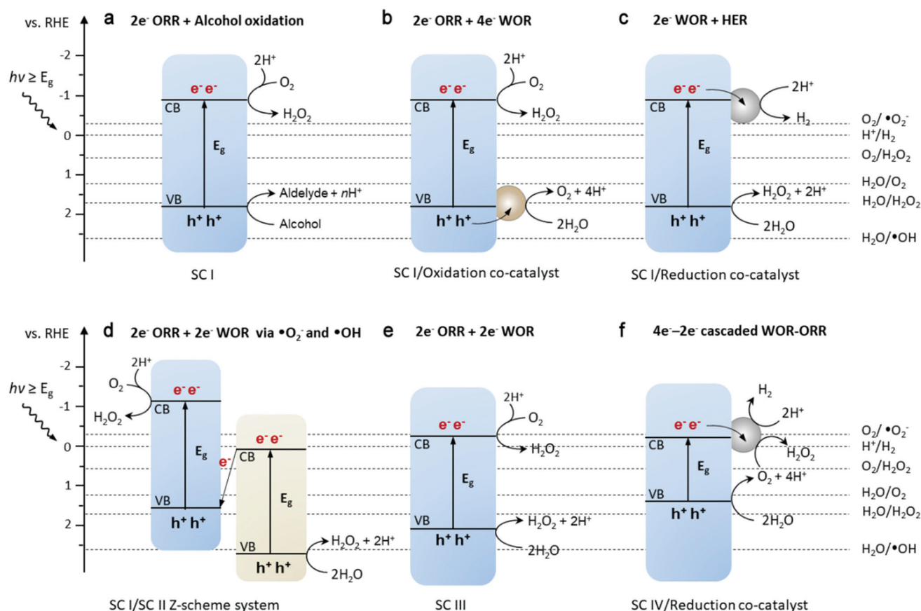
Fig. 5 Different redox pathways for photochemical H 2 O 2 formation (a–f) and selected redox reaction potentials regarding the oxygen reduction reaction (ORR) and water oxidation reaction (WOR). SC and HER are abbreviations of semiconductor and hydrogen evolution reaction, respectively. SCs I–IV are different semiconductors in previously reported specific systems for the photocatalytic synthesis of H 2 O 2 .
