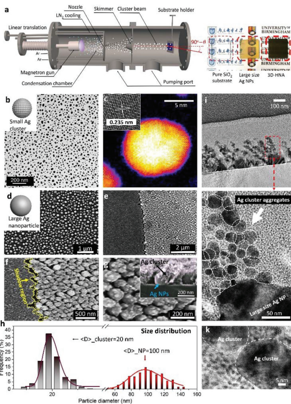
Fig. 2 (a) Left: Schematic illustration of the gas phase cluster beam deposition system. Right: Photographs of the blank SiO 2 substrate, large size Ag NP sample and 3D-HNA sample. (b) TEM image of Ag clusters generated from the cluster deposition system. (c) Typical HAADF-STEM image of a single Ag cluster. The inset is the HR-STEM image of the Ag cluster and the corresponding lattice constant has been marked in the figure. (d) SEM image of large size Ag NPs from the solid-state film dewetting process. (e) A typical SEM image of Ag cluster assemblies (left part) and 3D-Ag-HNA (right part). (f) A high magnification SEM image of Ag cluster assemblies (left part) and 3D-Ag-HNA (right part), the shadowing region has been marked in the figure. The inset shows a typical cross-sectional SEM image of 3D-Ag-HNA. (g) A high magnification SEM image of 3D-Ag-HNA. The inset shows a high magnification cross-sectional SEM image of 3D-Ag-HNA. (h) Size distribution of the Ag nanoparticles in the 3D-Ag-HNA and the corresponding log-normal fits. (i) TEM image of 3D-Ag-HNA. (j) A high magnification cross-sectional TEM image of a single unit in the 3D-Ag-HNA structure. (k) A high magnification TEM image of two Ag nanoclusters in the aggregate.
