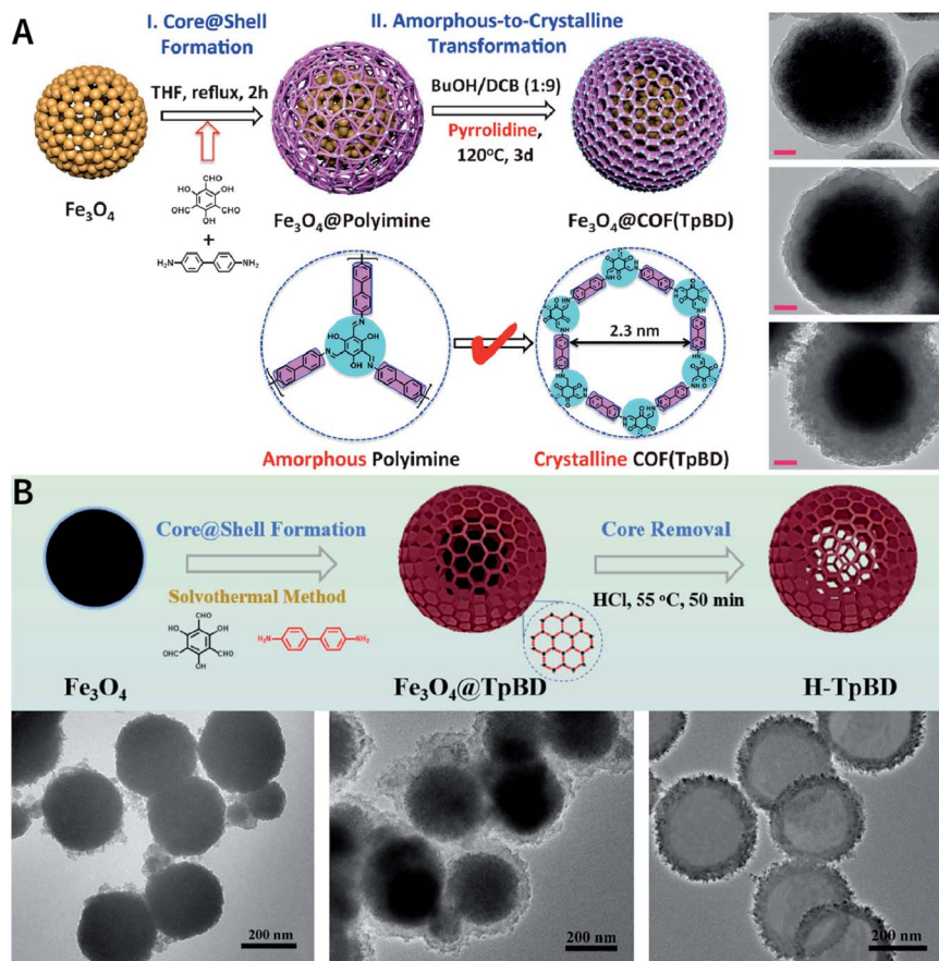
Fig. 38 (A) Preparation protocol and HRTEM images of Fe 3 O 4 @COF(TpBD) with shell thicknesses of 20, 50, and 100 nm. Scale bar: 50 nm. Adapted with permission. 232 Copyright 2016, Wiley-VCH Verlag GmbH & Co. KGaA, Weinheim. (B) Synthesis protocol and HRTEM images of hollow COF nanoshells. Adapted with permission. 233 Copyright 2018, Elsevier B.V.
