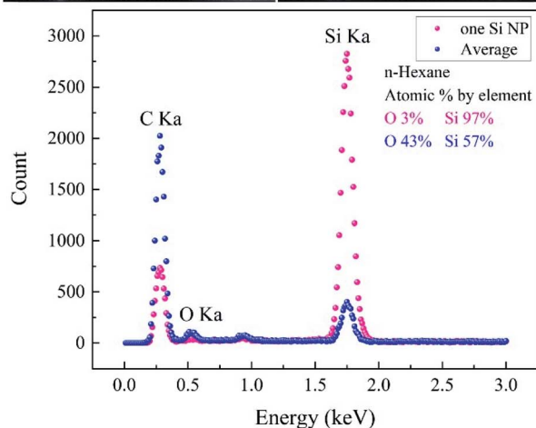
Fig. 7 The femtosecond laser-synthesized Si nanoparticles in n -hexane. ( N = 1000 , F = 10.46 \text{ J cm}^{-2} ). The TEM bright-field image, SAED pattern (upper right) and dark-field images related to different diffracted electron beams along the 1 st and 2 nd ring. The EDX spectrum from several small Si NPs and one Si NP.
