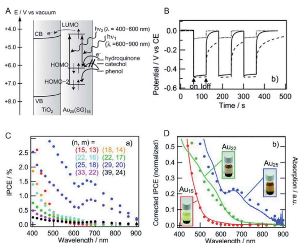
Fig. 12 (A) Mechanism of Au NCs sensitized solar cells. (B) Photopotential and (C) incident photons conversion efficiency (IPCE) spectra of Au NCs sensitized solar cells. (D) Normalized IPCE spectra and absorption spectra of Au NCs sensitized solar cells. Panels (a)–(d) are reproduced with permission from ref. 69. Copyright 2010 Wiley-VCH.
