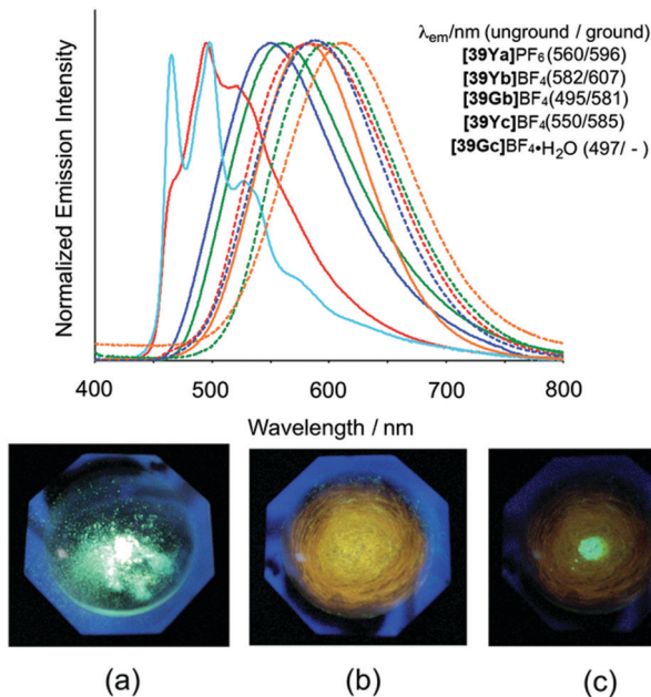
Fig. 15 Top: Normalized emission spectra of the Pt II based complexes in the solid state at 295 K ( \lambda_{\text{ex}} = 365 nm). Solid and dashed lines correspond to the spectra of unground and ground samples, respectively. Bottom: Photographic images of [39Gb]BF 4 in response to mechanical grinding under UV light irradiation (365 nm): (a) unground sample, (b) completely ground sample, (c) ground sample with a drop of acetonitrile. Reprinted with permission from ref. 57. Copyright 2014 Royal Society of Chemistry.
