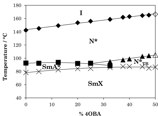
Fig. 4 Dependence of phase behaviour of the 1OB6OS:4OBA:(S)-(2-Me)4OBA series of ternary mixtures on the molar percentage of achiral H-bond donor 4OBA, where \diamond represents T_{N^*I} , \blacksquare T_{SmA^*N^*} , \blacktriangle T_{N^*TB}N^* and \times T_{NTB/SmA-SmX} . Unfilled diamond and triangle represent conventional N-I and N_{TB}-N , respectively. Melting points omitted for clarity.
