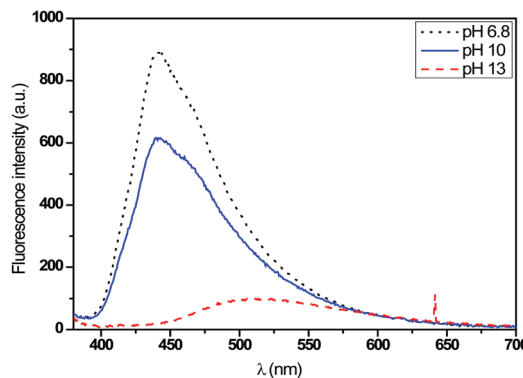
Fig. 13 Emission spectrum of the T3 fabric as a function of pH under excitation at 365 nm.
