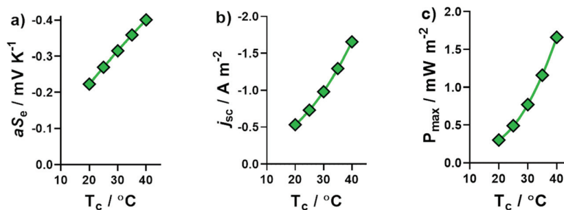
Fig. 4 Plots showing the significant effect different applied T_c values have upon the thermogalvanic properties of the [\text{Fe}(\text{SO}_4)_2]^{-/-} system, as quantified by the (a) aS_e , (b) j_{SC} , and (c) P_{max} . For all measurements \Delta T = 10 K, applied T_h = T_c + 10 °C, and applied T_c is indicated by the x-axis. Second order polynomial lines of best fit have been added to guide the eye of the reader, and are not intended to model the data.
