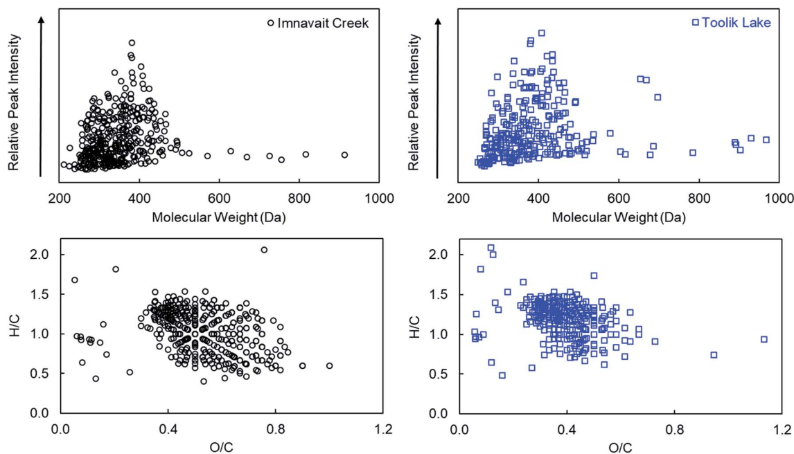
Fig. 2 Molecular-level compositional characteristics of ^{18}\text{O} -containing products after exposing Innavait Creek (black circles) and Toolik Lake DOM (blue squares) to sunlight. Top: molecular weight vs. relative peak intensity of ^{18}\text{O} photo-products. Bottom: van Krevelen plots of ^{18}\text{O} photo-products.
