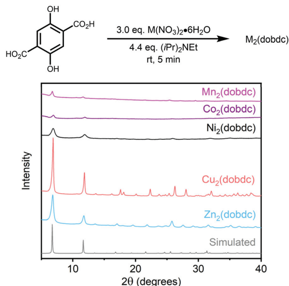
Fig. 5 Powder X-ray diffraction patterns ( \lambda = 1.5406 \text{ \AA} ) of M 2 (dobdc) (M = Mn, Co, Ni, Cu, Zn) prepared under mechanochemical conditions. The simulated pattern based on the previously reported single-crystal X-ray diffraction structure of the framework Zn 2 (dobdc) is included for reference. 53
