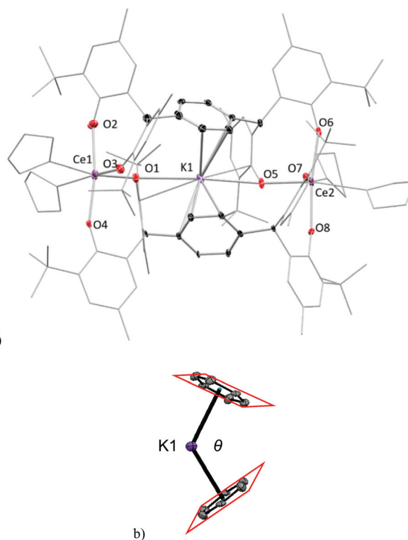
Fig. 2 Solid state structure of complex 2 Me . (a) core of anion with K(THF) 7 counter-cation and all H and two lattice THF solvent molecules omitted for clarity. Coordinated solvent shown as wireframe, and ligands shown as capped stick for clarity; thermal ellipsoids of other atoms are shown at 30% probability. (b) Bis(η 6 -arene) coordination of the endo K + cation with the angle between the two arene planes labelled as θ.
