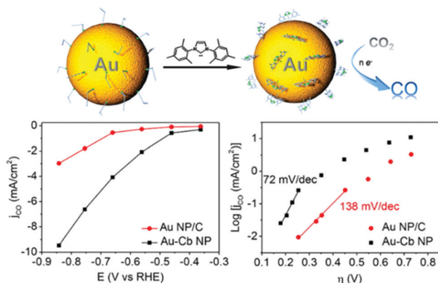
Fig. 35 Schematic illustration of NHC-carbene functionalized Au NPs for CO 2 RR to CO. Partial current density and Tafel plot for CO 2 RR to CO for Au–Cb NP and Au NP/C. Reproduced with permission from ref. 454. Copyright 2016 American Chemical Society.
