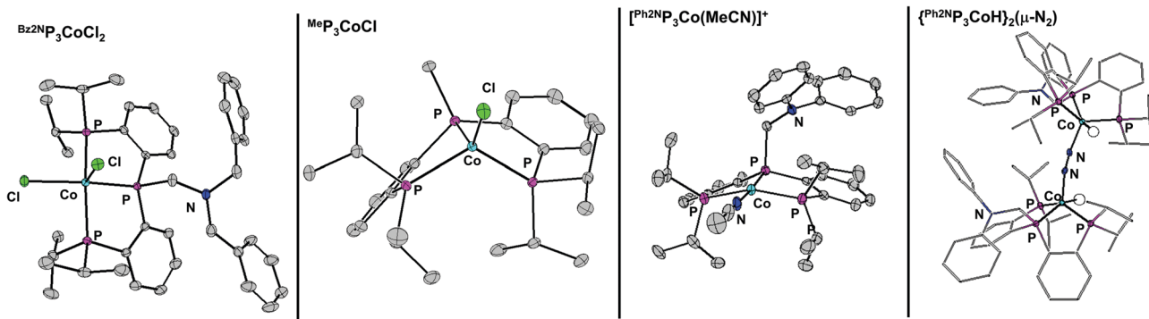
Fig. 1 50% thermal ellipsoid plot of several complexes. All hydrogen atoms not located in the difference map are removed for clarity. Only the cation of [(\text{Ph}_2\text{N}^{\text{R}'\text{R}''}\text{P}_3)\text{Co}(\text{MeCN})][\text{BARf}]^+ is shown.
