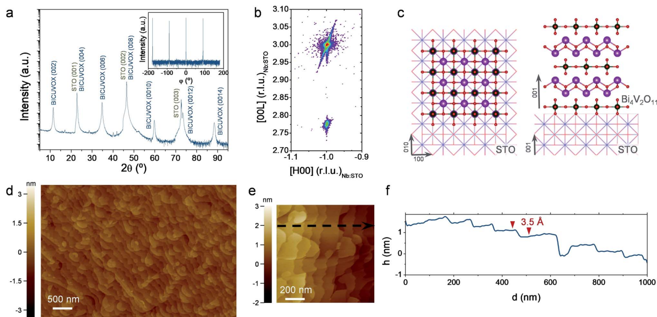
Fig. 2 (a and b) X-ray diffraction patterns of a 36 nm thick BICUVOX film deposited on Nb-doped SrTiO 3 . (a) Out-of-plane 2\theta X-ray diffraction pattern, where the set of peaks corresponding to the 00L reflections is visible. A \phi scan around the (–103) reflection of SrTiO 3 is also included in the inset, showing a 4-fold symmetry corresponding to a single in-plane orientation (100) BICUVOX/(100) SrTiO 3 . (b) Shows the in-plane Reciprocal Space Map around the –103 reflection peak of the Nb-doped SrTiO 3 substrate. (c) Schematic representations of the epitaxial growth of \gamma -Bi 4 V 2 O 11 on top of 001-oriented SrTiO 3 single crystals, top and cross-sectional views. (d and e) AFM images of an epitaxial BICUVOX film grown on top of Nb-doped SrTiO 3 , with two different magnifications. (f) Height profile corresponding to the black dashed arrow shown in figure (e). The average step height is shown as well (only single step terraces are considered for the average calculation).
