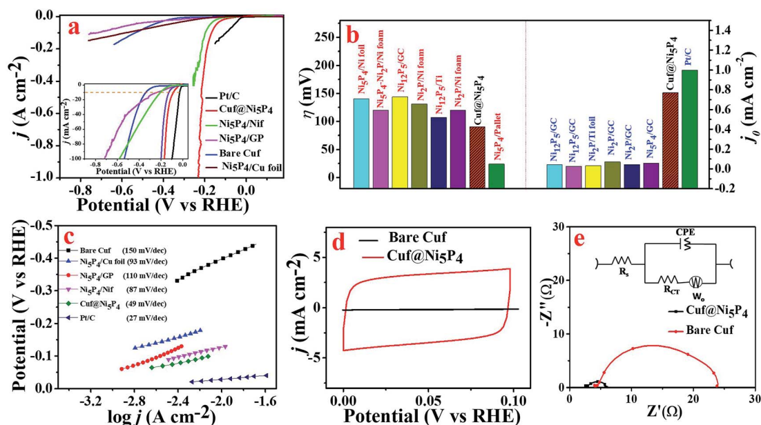
Fig. 5 (a) HER polarization curves for bare Cu, \text{Ni}_5\text{P}_4/\text{Cu} foil, \text{Ni}_5\text{P}_4/\text{GP} , \text{Ni}_5\text{P}_4/\text{Nif} , \text{Cu}@\text{Ni}_5\text{P}_4 and Pt/C catalysts recorded at a scan rate of 10 \text{ mV s}^{-1} . (b) Bar diagram depicting the comparison of the overpotential and the exchange current density of the previously reported nickel phosphide based electrocatalyst. (c) Tafel plots of bare Cu, \text{Ni}_5\text{P}_4/\text{Cu} foil, \text{Ni}_5\text{P}_4/\text{GP} , \text{Ni}_5\text{P}_4/\text{Nif} , \text{Cu}@\text{Ni}_5\text{P}_4 and Pt/C. (d) CV response of bare Cu and \text{Cu}@\text{Ni}_5\text{P}_4 at a scan rate of 100 \text{ mV s}^{-1} . (e) Nyquist plot of bare Cu and \text{Cu}@\text{Ni}_5\text{P}_4 recorded at -0.2 \text{ V} (vs. RHE), the inset shows the equivalent circuit used to fit the EIS data. All of the experiments were performed in 0.5 M \text{H}_2\text{SO}_4 solution.
