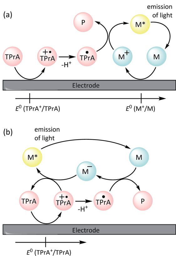
Scheme 1 Co-reactant ECL mechanisms involving (a) electrochemical oxidation the tri- n -propylamine co-reactant (TPrA) and metal complex (M; [Ru(bpy) 3 ] 2+ ), or (b) oxidation of the co-reactant only, 5,21 where TPrA •+ is an aminium radical cation, TPrA • is a neutral \alpha -amino alkyl radical, and P is its subsequent products. The additional 'catalytic route' involving oxidation of TPrA by M + , and an 'annihilation' pathway, in which the excited state is generated from the reaction of M + (from a) with M - (from b), are shown in Scheme S1 in the ESI.†
