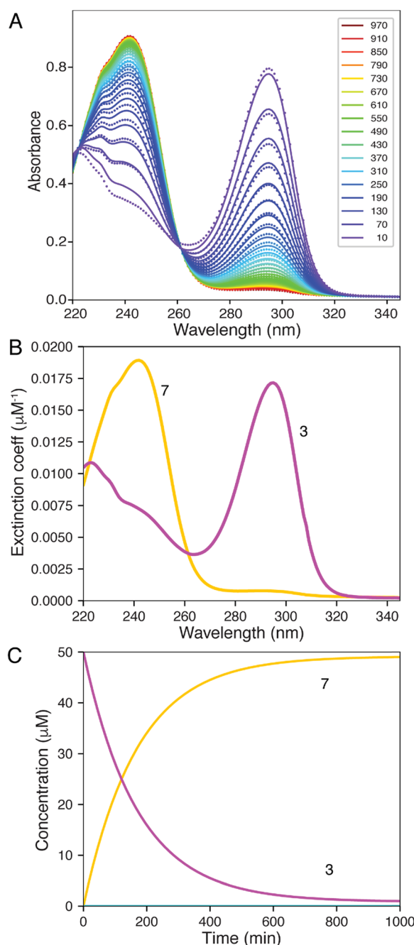
Fig. 3 (A) Time course for the UV-vis absorbance spectra of the reaction of 3 (50 \mu\text{M} ) to form 7 after being placed in a 2 : 1 H 2 O : MeOH mixture at pH 6.8. The dots show the experimental data, while the solid lines show the fitted curve. The peak at 240 nm increases while the peak at 295 nm decreases. (B) Spectra derived from fitting 3 , magenta; 7 , yellow. (C) Time dependence of conversion of 3 (magenta) to 7 (yellow).
