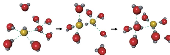
Fig. 9 Schematic illustration of the migration of OH^- ions with water molecules in the water solvent. Reproduced from ref. 51 with permission from Nature Publishing Group, Copyright 2002.
