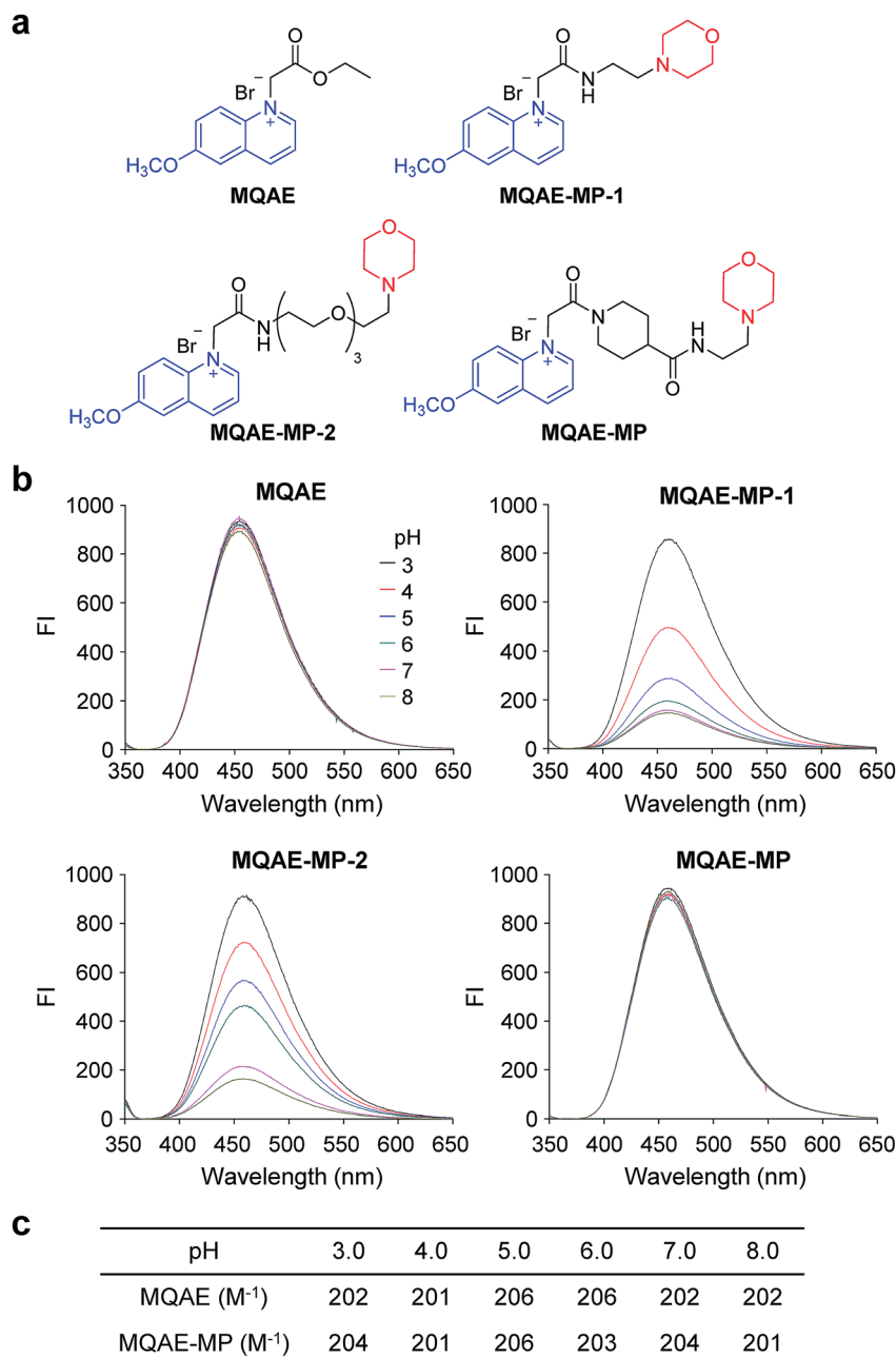
Fig. 1 Effect of pH on the fluorescence emission of the fluorescent Cl^{-} probes. (a) Chemical structures of the fluorescent Cl^{-} probes. (b) Fluorescence spectra of each probe (100 \mu M ) in 50 mM sodium phosphate buffer at pH 3.0–8.0 were recorded on a fluorimeter with excitation at 350 nm wavelength (FI = fluorescence intensity). (c) Stern–Volmer constants for quenching of the fluorescence of MQAE and MQAE-MP by Cl^{-} at various pHs.
