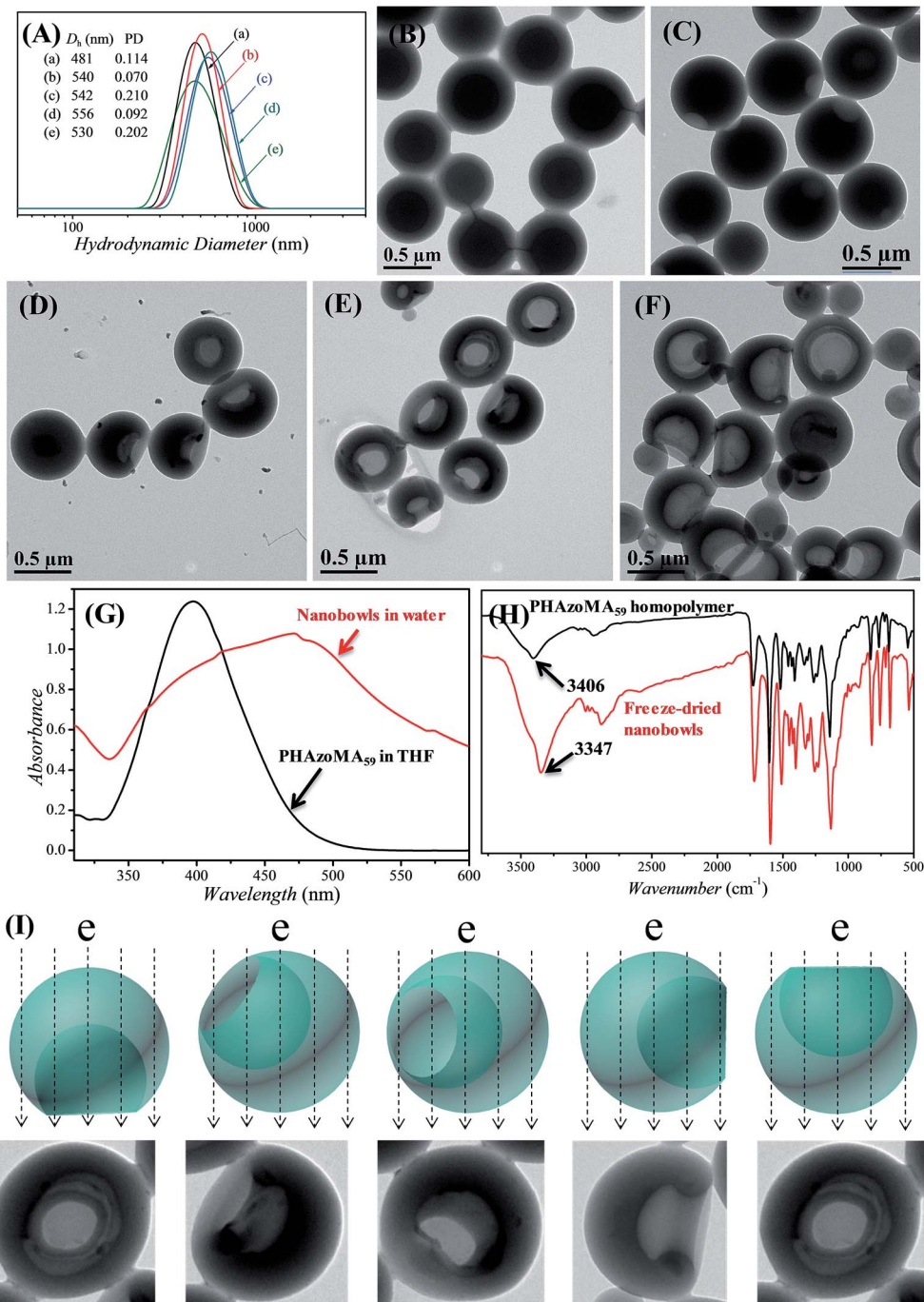
Fig. 1 Evolution from PHAzO MA -based homopolymer complex micelles (HCMs) to nanobowls. (A) DLS results of the corresponding nanostructures when the DPs of PHAzO MA are (a) 10, (b) 29, (c) 59, (d) 116 and (e) 226, respectively; (B) TEM images of HCMs when the DP is 10; (C), (D), (E) and (F) TEM images of nanobowls with different sizes of openings and interior holes when the DPs are 29, 59, 116 and 226, respectively; (G) UV-vis spectra of PHAzO MA 59 in THF and nanobowls in water, with the red shift of the absorption peak of nanobowls indicating the \pi - \pi interaction between azobenzene moieties after self-assembly; (H) FT-IR spectra of PHAzO MA 59 and freeze-dried nanobowl powder, with the expanding and the shift of the absorption peak of -OH to a lower wavenumber indicating the formation of hydrogen bonds in nanobowls; (I) images representing the diverse morphologies of nanobowls in TEM images due to different presentation angles.
