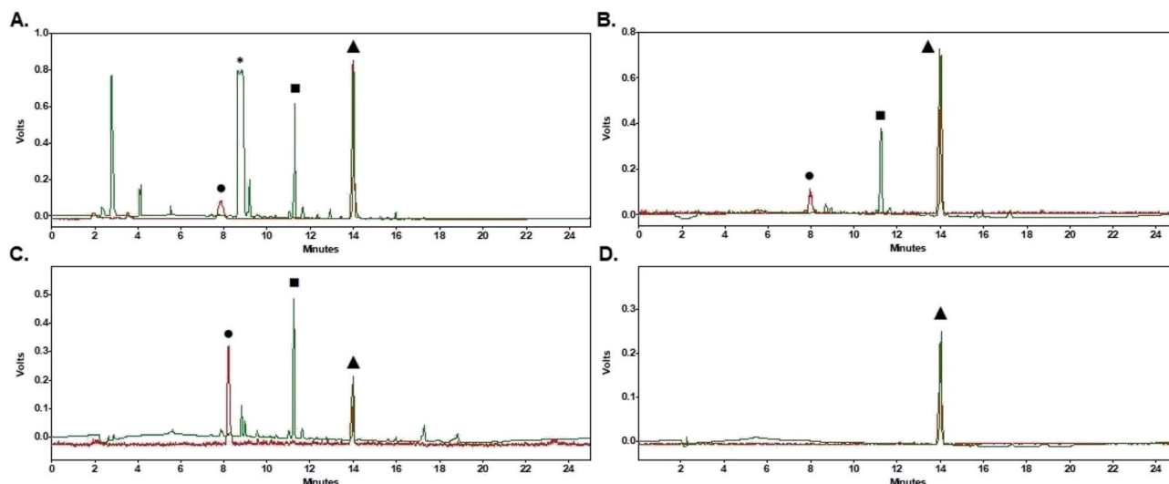
Fig. 5 [^{18}\text{F}] FPy-TFP (5) HPLC-chromatograms (PMT (gamma)-red, UV (220 nm)-green). (A) Crude HPLC chromatogram (peak ● - [^{18}\text{F}] fluoronicotinic acid, peak * -PyTFP-precursor (4), peak ■ -2,3,5,6-tetrafluorophenol (9), peak ▲ - [^{18}\text{F}] FPy-TFP (5)). (B) HPLC chromatogram after MCX-cartridge purification (peak ● - [^{18}\text{F}] fluoronicotinic acid, peak ■ -2,3,5,6-tetrafluorophenol (9), peak ▲ - [^{18}\text{F}] FPy-TFP (5)). (C) HPLC chromatogram after MCX-C18SepPak double cartridge purification (peak ● - [^{18}\text{F}] fluoronicotinic acid, peak ■ -2,3,5,6-tetrafluorophenol (9), peak ▲ - [^{18}\text{F}] FPy-TFP (5)). (D) Purified HPLC-chromatogram co-injected with [^{19}\text{F}] FPy-TFP (peak ▲ - [^{18}\text{F}] FPy-TFP (5)).
