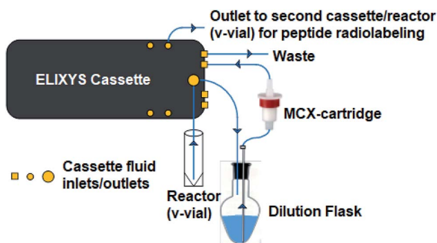
Fig. 3 Diagram of gross dilution set-up. Set-up allows [ ^{18}F ]FPy-TFP (5) purification via a 15 mL water dilution in an external flask, trapping on an Oasis MCX cartridge followed by a 5 mL water wash and 3 mL acetonitrile elution. All operations are fully automated via ELIXYS FLEX/CHEM® radiosynthesizer and no manual interventions required.
