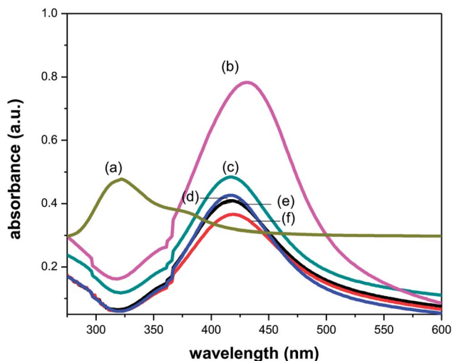
Fig. 3 UV-vis absorption spectra of (a) amikacin, (b) PVP-AgNPs, (c–f) Amk@PVP-AgNPs at concentration 0.05 , 0.1 , 0.3 and 0.5 \text{ mM} respectively.
