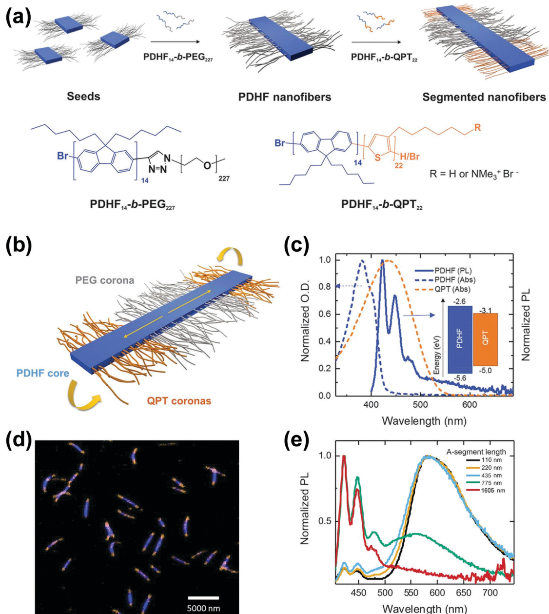
Fig. 6 (a) Schematic illustration of the seeded growth process and the molecular structures of \text{PDHF}_{14}\text{-}b\text{-PEG}_{227} and \text{PDHF}_{14}\text{-}b\text{-QPT}_{22} . (b) The segmented B-A-B nanofiber structure with separate donor and acceptor domains. (c) Normalized absorption of QPT homopolymer in THF : MeOH (1 : 1) (orange dashes), and unsegmented PDHF nanofibers (blue dashes), and photoluminescence (PL) emission of unsegmented PDHF nanofibers in the same solution (solid blue line). The inset shows the energy levels of the PDHF and QPT. (d) Laser scanning confocal microscopy (LSCM) image of the uniform segmented PDHF nanofibers with a crystalline PDHF core (blue emission) and two terminal blocks with QPT coronas (orange emission). (e) Normalized PL spectra of segmented PDHF nanofibers with different A-segment lengths. Emission arising from direct excitation of the QPT in the 1605 nm sample was unresolved. Reproduced with permission from ref. 50. Copyright 2018, American Association for the Advancement of Science.
