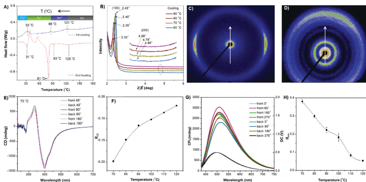
Fig. 5 (A) DSC thermograms of DPCE-ECh recorded at the second heating and first cooling scans ( 5\text{ }^\circ\text{C min}^{-1} ). Inset: Phase transition of DPCE-ECh determined from the first cooling DSC scans at a rate of 5\text{ }^\circ\text{C min}^{-1} . (B) 1D WAXD pattern of DPCE-ECh recorded in the first cooling process at a temperature of 60–90 °C. ( 2\theta = 2^\circ\text{--}6^\circ , inset: high-order diffractions). (C) 2D SAXS and (D) 2D WAXS patterns of the mechanically aligned DPCE-ECh with X-ray beam perpendicular to the shear direction. (E) CD spectra (404 nm) of front and back sides of DPCE-ECh films annealed at 70 °C recorded for 45 min at different rotation angles perpendicular to the light axis. The film thickness is 50 nm for CD detection. (G) g_{lum} (510 nm) of front and back sides of DPCE-ECh films annealed at a temperature of 70 °C for 45 min at different rotation angles perpendicular to the light axis. The film thickness is 7 \mu m for CPL detection. (F and H) g_{CD} and g_{lum} of DPCE-ECh at different temperatures.
