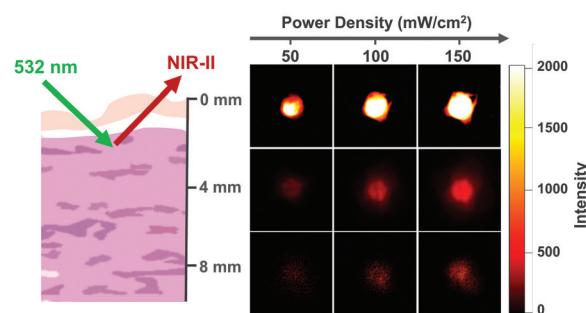
Fig. 2 Luminescence intensity of Yb-2 ( 2 \text{ mg mL}^{-1} ) in the NIR-II region (100 ms exposure, 1000 nm longpass filter) under the corresponding penetration depth (0, 4 and 8 mm) and excitation laser power (532 nm, 50, 100 and 150 \text{ mW cm}^{-2} ).
