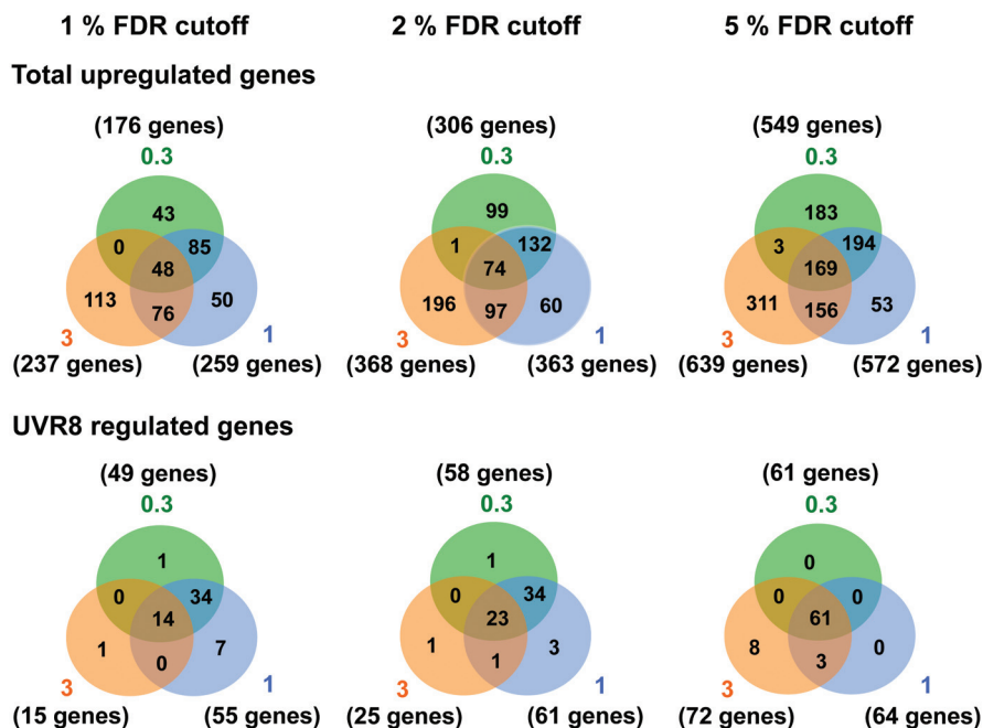
Fig. 1 Venn diagrams depicting the overlap in gene expression at different fluence rates of UV-B. Three-week-old Arabidopsis plants grown in a low fluence rate of white light ( 20 \mu\text{mol m}^{-2} \text{s}^{-1} ) were treated with either 4 hours of 0.3 , 1 or 3 \mu\text{mol m}^{-2} \text{s}^{-1} broadband UV-B or were left in low white light as a control. This corresponds to a plant weighted \text{UV}^{51} of 0.08 , 0.27 , and 0.82 \text{ kJ m}^{-2} , respectively, which compares with 4.8 \text{ kJ m}^{-2} \text{ day}^{-1} in Lund, Sweden, at midsummer under a cloudless sky. 51 The numbers of genes that showed an increase in transcript level were calculated for each of three False Discovery Rates (FDR). Gene lists were then compared to those published by Brown et al. (2005) 18 to determine overlap and dependence on UVR8. Numbers in orange circles denote transcripts identified in the Brown et al. (2005) 18 3 \mu\text{mol m}^{-2} \text{s}^{-1} UV-B microarray, those in blue and green are those found in this study to be induced by 1 and 0.3 \mu\text{mol m}^{-2} \text{s}^{-1} UV-B respectively.
