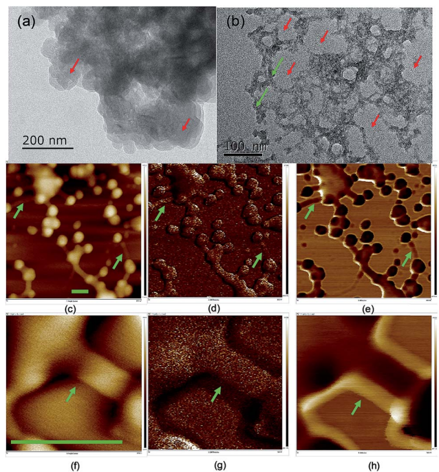
Fig. 2 TEM images of the carbon dots before (a) and after (b) ageing. AFM images of the carbon dots on a silicon single crystal after eight months of ageing in terms of height (c, f), Young's modulus (d, g) and adhesion (e, h) at different magnifications. The scale bars in (c–h) represent 100 nm and the green arrows indicate the floccs binding the carbon dots while the red arrows indicate the carbon dots. (f–h) are images highlighting the morphology of the floccs connecting the particles.
