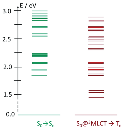
Fig. 7 TD-DFT excited state calculations for Fe II (btz) 3 . Shown excitations include singlet excitations at SO geometry (left, green), and triplet excitations from the SO state at the 3 MLCT geometry (right, red). Energies and assignments from Chábera et al. 39
