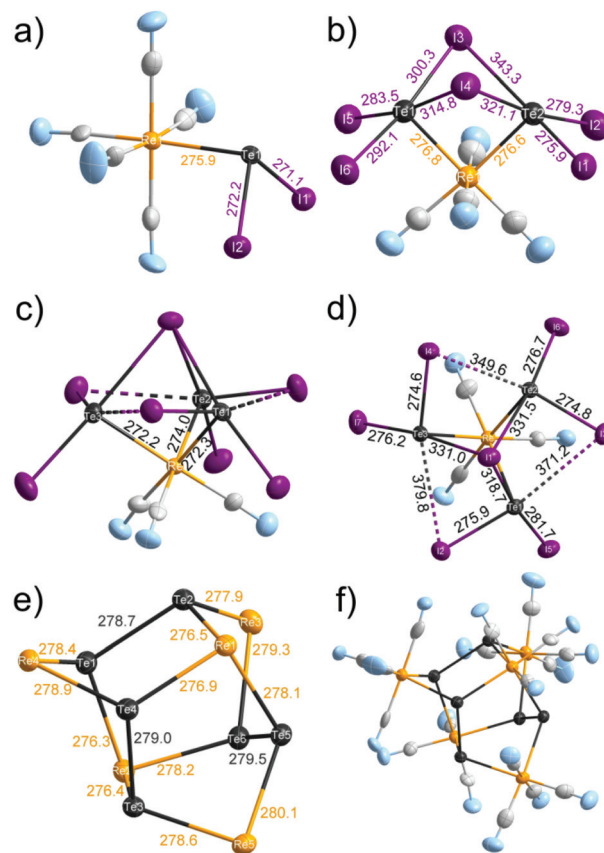
Fig. 2 Structural units and connectivity of the Te–Re carbonyls with selected bond distances (in pm; Te–Te: black, Te–I: violet, Te–Re: yellow): (a) [\text{Te}_2\text{Re}(\text{CO})_5]^+ cation in 1; (b) [\text{Te}_2\text{I}_4(\mu\text{-I})_2\text{Re}(\text{CO})_4]^- anion in 2; (c, d) \{\text{Te}_3\text{I}_2(\mu\text{-I})_3(\mu_3\text{-I})\}\text{Re}(\text{CO})_4 (3) with structure of (c) rotated by 90° in (d); (e) \text{Te}_6\text{Re}_5 unit in 4; (f) [(\text{Te}_2)_3\{\text{Re}(\text{CO})_3\}_2\{\text{Re}(\text{CO})_4\}_3]^- anion in 4.
