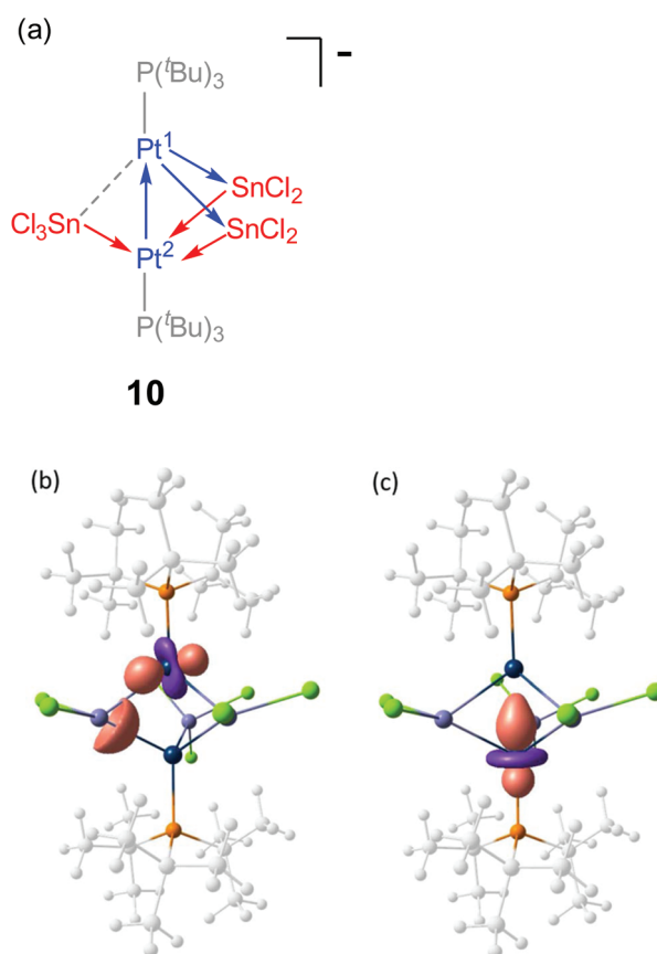
Fig. 6 (a) Simplified bonding scheme representation of compound 10 , where arrows describe electron donation between metal centres; (b, c) Representative localized molecular orbitals (Pipek–Mezey) involved in the Pt–Sn (b) and the Pt–Pt bonding (c).
