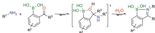
Fig. 15 Strategies for amine condensation with carbonyl compounds. (A) Imine formation, reversibility in aqueous media and reductive amination. (B) Iminoboronate formation and reversibility in aqueous media.
