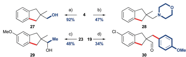
Scheme 3 Derivatisation of indane products. (a) NaBH 4 , MeOH, 2 h 0–25 °C, (b) morpholine, NaBH(OAc) 3 , CH 2 Cl 2 , 25 °C, 24 h. (c) MeMgCl, Et 2 O, 0–25 °C, 1.5 h. (d) TDG1 (50 mol%), 4-iodoanisole, Pd(OAc) 2 (5 mol%), AgTFA, DMSO (1 equiv.), HFIP:AcOH (1:1), 130 °C, 3 h. Product isolated as a 5.7:1 mixture with a 4-acetoxyanisole by-product.
