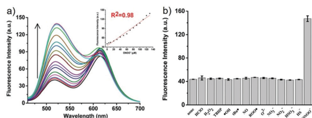
Fig. 105 (a) The fluorescence spectra of 64 (5 \mu\text{M} ) in the presence of different concentrations of \text{ONOO}^- (0–150 \mu\text{M} ) in \text{H}_2\text{O} : ethanol (5:5 v/v) containing 0.5% DMSO (pH = 5.0), and 10 mM CPBS at room temperature. The insert shows the plot of fluorescence intensity at 510 nm versus various concentrations of \text{ONOO}^- . The excitation wavelength = 440 nm, excitation and emission slit widths were both 5 nm. Each spectrum was acquired 3 min after \text{ONOO}^- addition at room temperature. (b) Fluorescence intensity of 64 (5 \mu\text{M} ) at 510 nm in the presence of \text{ONOO}^- (150 \mu\text{M} ) and various ROSs (200 \mu\text{M} ), \text{HSO}_3^- (200 \mu\text{M} ), \text{HS}^- (200 \mu\text{M} ), \text{NO}_3^- (200 \mu\text{M} ), \text{NO}_2^- (200 \mu\text{M} ). Excitation wavelength = 440 nm, excitation and emission slit widths were both 5 nm. Each spectrum was acquired 10 min after the addition of the various ROSs and RNSs at room temperature. Copyright 2018 Royal Society of Chemistry.
