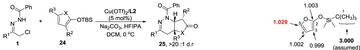
Scheme 11 Carbon isotope effects ( R/R_0 ) calculated for TBSO furan. The three methyl carbons of the tBu group (in bold) were taken as the internal standard.
