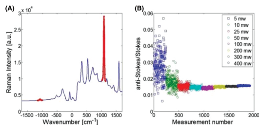
Fig. 1 (A) Raman spectrum of Au-MBA nanoparticles alone deposited on \text{CaF}_2 with the ( 1085\text{ cm}^{-1} \nu_{12} benzene ring mode) highlighted in red. (B) anti-Stokes/Stokes intensity ratio ( \nu_{12} benzene ring mode) of MBA labelled gold nanoparticles alone deposited on \text{CaF}_2 measured between 5–400 mW at 830 nm excitation.
