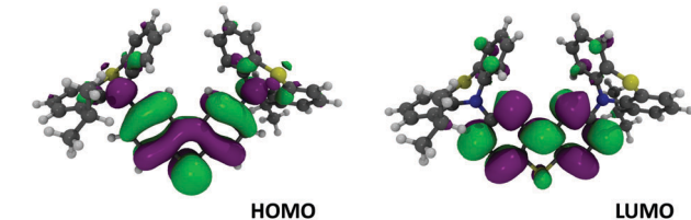
Fig. 4 Molecular orbitals, HOMO and LUMO of DPTZ-DBT (equatorial) and DPTZ- i Pr-DBT (axial) forms at DFT (M062X)/Def2SVP level of theory.
