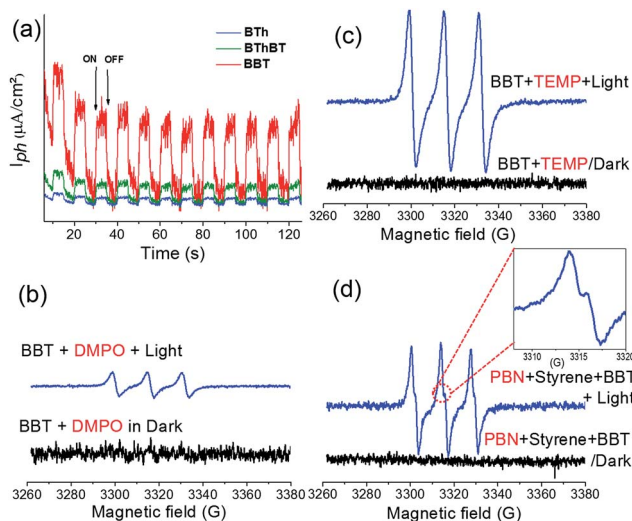
Fig. 4 (a) Photocurrent responses of the CMPs under the illumination of visible light with a wavelength \geq 420 nm with light ON/OFF model. EPR spectra of (b) DMPO- \text{O}_2^{\bullet -} ( g = 2.00639 ) and (c) TEMP- ^1\text{O}_2 adducts ( g = 2.00645 ) using BBT as the photocatalyst in the dark and under light irradiation ( \lambda = 460 nm, 0.065 W \text{cm}^{-2} ). (d) EPR spectra using PBN as a radical trapping agent for the radical intermediate of styrene, with BBT, under \text{O}_2 and light irradiation ( g = 2.00667 ).
