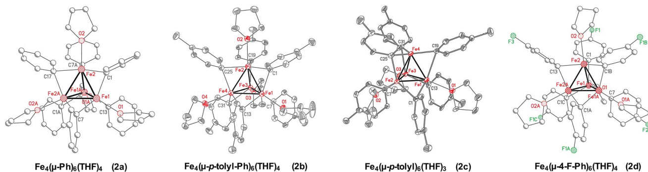
Fig. 3 Crystal structures of the tetranuclear iron–aryl clusters, with hydrogen atoms omitted for clarity. Due to weakly diffract crystals, the structures of \text{Fe}_4(\mu\text{-Ph})_6(\text{THF})_4 ( 2a ) and \text{Fe}_4(\mu\text{-4-F-Ph})_6(\text{THF})_4 ( 2d ) are used solely for connectivity and chemical formulation as shown. For structures with p -tolyl groups, \text{Fe}_4(\mu\text{-}p\text{-tolyl})_6(\text{THF})_3 ( 2b ) and \text{Fe}_4(\mu\text{-}p\text{-tolyl})_6(\text{THF})_4 ( 2c ), adequate intensity data could be obtained and the ellipsoids are shown at 50% probability.
