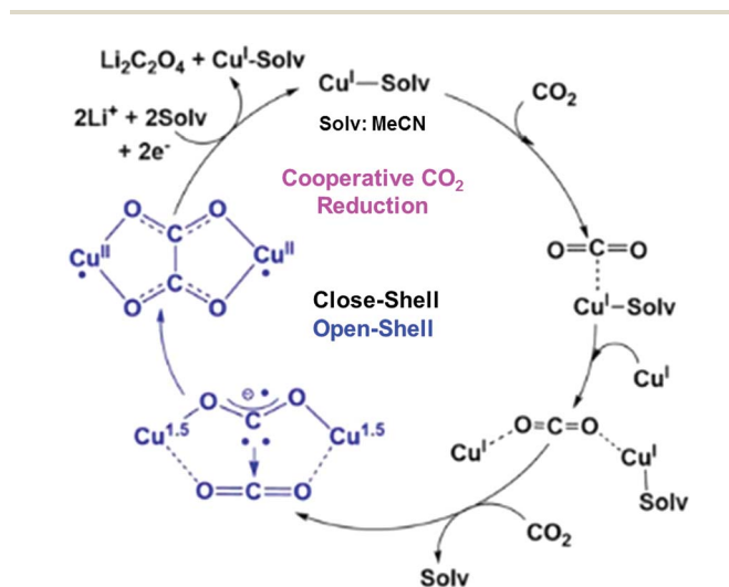
Scheme 2 Proposed catalytic cycle for one-electron reduction of \text{CO}_2 to oxalate with a copper(I) complex. Reprinted with permission from ref. 79. Copyright 2017, American Chemical Society.
