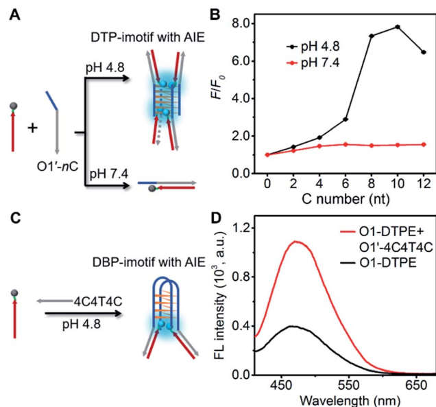
Fig. 6 (A) Schematic illustration of the DTP-imotif structure adopted at pH 4.8 and the double-stranded structure formed at pH 7.4. (B) Ratios of fluorescent peak intensity of 1.0 \mu\text{M} O1-DTPE after and before ( F/F_0 ) hybridization with O1'- n\text{C} ( n = 0 to 12) in pH 4.8 TAE reaction buffer and in pH 7.4 TE reaction buffer at 25 ^\circ\text{C} . (C) Schematic illustration of the DBP-imotif structure. (D) Fluorescence spectra of 1.0 \mu\text{M} O1-DTPE and the mixture of 1.0 \mu\text{M} O1-DTPE and O1'-4C4T4C in pH 4.8 TAE reaction buffer at 25 ^\circ\text{C} .
