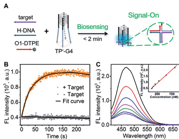
Fig. 7 (A) Schematic illustration of the DNA detection strategy that relies on the self-assembly of four-way junctions. (B) Time-dependent fluorescence signal for 1.0 \mu\text{M} O1-DTPE, 1.0 \mu\text{M} H-DNA, and 1.0 \mu\text{M} TP'-G4-5 bp in the presence and absence of target DNA in TE reaction buffer at 25 ^\circ\text{C} . (C) Fluorescence spectra of 1.0 \mu\text{M} O1-DTPE after mixing with 1.0 \mu\text{M} H-DNA and TP'-G4 in the presence of target DNA at different concentrations for 1.5 min in TE reaction buffer at 25 ^\circ\text{C} . Inset is the calibration curve.
