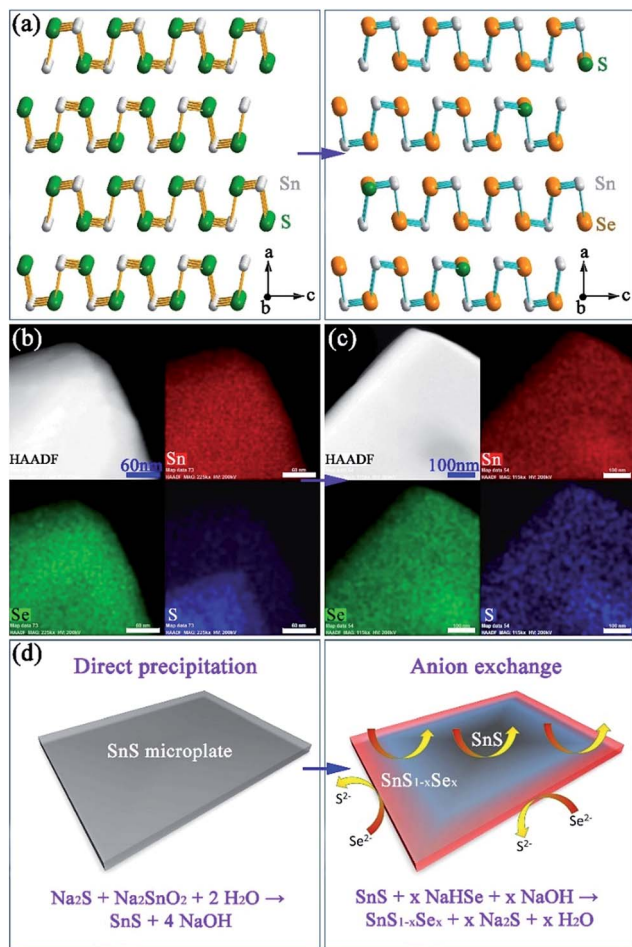
Fig. 3 Structure, composition and formation mechanism of \text{Sn}(\text{S,Se}) : (a) structural models of SnS and \text{SnS}_{1-x}\text{Se}_x ; elemental mapping of isolated plates after anion exchange for (b) 1 min and (c) 2 h; (d) schematics of the initial precipitation and subsequent exchange processes. The four panels in (b) and (c) show the high angle annular dark field (HAADF) image of a plate and corresponding elemental maps for Sn (red), Se (green) and S (blue) respectively.
