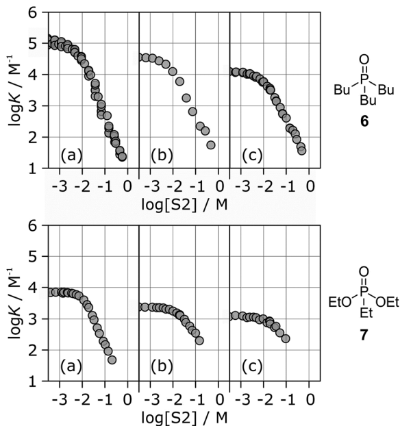
Fig. 6 Association constants ( \log K/M^{-1} ) for formation of 1:1 complexes between H-bond acceptor 6 (upper row) or 7 (lower row) and different H-bond donors as a function of concentration of 1-octanol (S2) in n -octane (S1) at 298 K. Donors are (a) 13, (b) 14, (c) 15.
