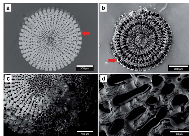
Fig. 2 SEM images of (a) the sea urchin spine template and (b) the synthesised PPy. The PPy structure is equal to a coating of the original \text{CaCO}_3 structure. This can be easily realised at the outer part marked with the red arrows. (c) and (d) show SEM images of the composite material consisting of \text{CaCO}_3 from the sea urchin spine and PPy. The \text{CaCO}_3 has been dissolved partly in this sample. (c) The light structures of \text{CaCO}_3 can be seen. They are surrounded by a layer of PPy. The dark part of the structure is the remaining PPy where the \text{CaCO}_3 has been dissolved already. (d) The image shows the inner part of the braces which are partly dissolved and a layer of PPy around the surface of the braces.
