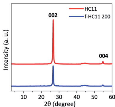
Fig. 6 XRD pattern of the pristine HC11 and f-HC11 200.
