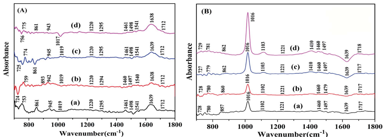
Fig. 9 (A) The difference spectra of free DNA (a) and [(DNA + TBZ) – TBZ]. (B) The difference spectra of free drug (a) and [(DNA + TBZ) – DNA]. The molar ratios ([TBZ] : [hsDNA]) for (b)–(d) were 1 : 20, 1 : 40 and 1 : 80, respectively.
