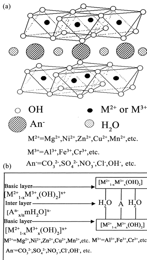
Fig. 1 Structure models for LDHs [\text{M}_{1-x}^{2+}\text{M}_x^{3+}(\text{OH})_2][\text{A}^{n-}]_{x/n} \cdot m\text{H}_2\text{O} (a) 3D structure and (b) 2D structure (reproduced with permission from ref. 68).
