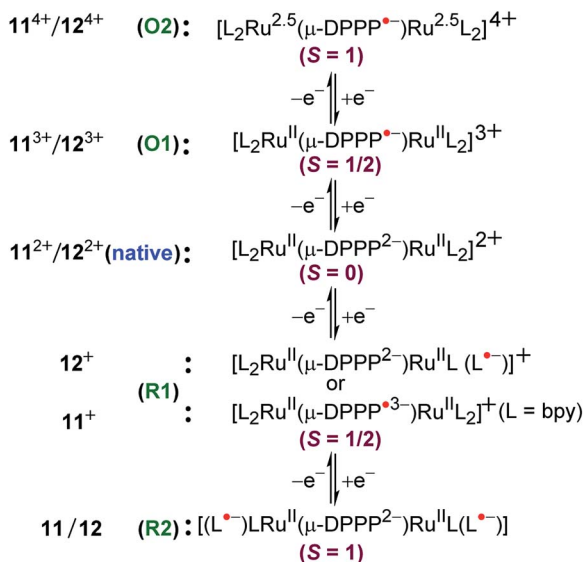
Fig. 13 Electronic structural forms of 11^{\cdot} and 12^{\cdot} .
