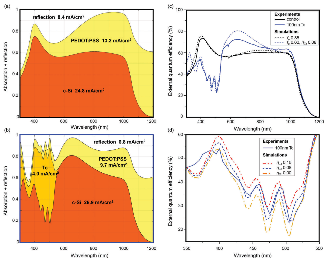
Fig. 4 The optical absorption data of a simulated control device (a) and 100 nm Tc device (b) generated using GenPro4. 74 Current densities are calculated for each device layer, including reflections to air. Model EQE spectra in (c) were constructed using the optical data in (a) and (b) folded with an internal quantum efficiency for the each active layer. The best fit to the measured 100 nm Tc spectrum is obtained for \eta_{\text{Tc}} = 0.08 , suggesting some exciton harvesting is occurring. A detailed view of the Tc absorption region is shown in (d); alongside the two spectra from (a) there are two otherwise-identical simulations with \eta_{\text{Tc}} of 0 and 0.16. The fit is consistent with a non-zero yield of exciton harvesting from Tc.
